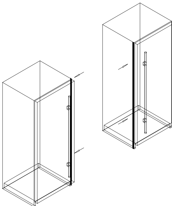
6 Install the adhesive fixed bar Installer la barre fixe adhésive
